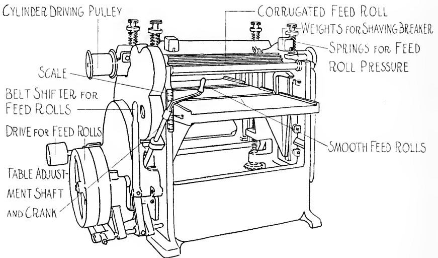
FIG. 152. PLANER OR SURFACER.
